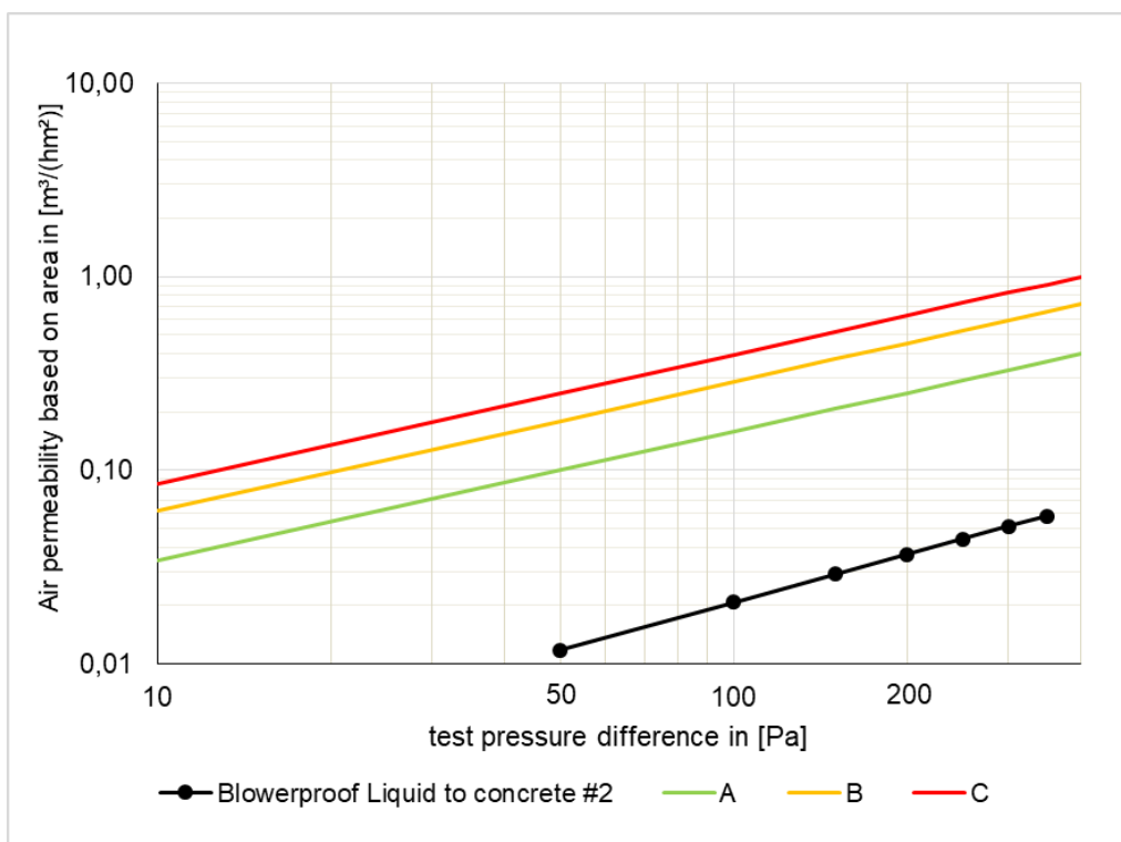
Fig. 13: Series of measurements for the sample "Blowerproof Liquid/concrete #2"... The Certification Classes A to C according to the PHI are entered in addition.
