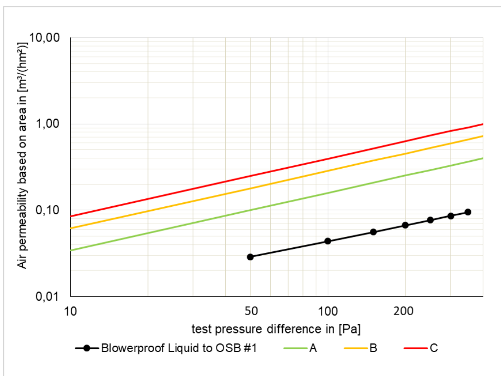
Fig. 9: Series of measurements for the sample "Blowerproof Liquid/OSB #1". The Certification Classes A to C according to the PHI are entered in addition.
