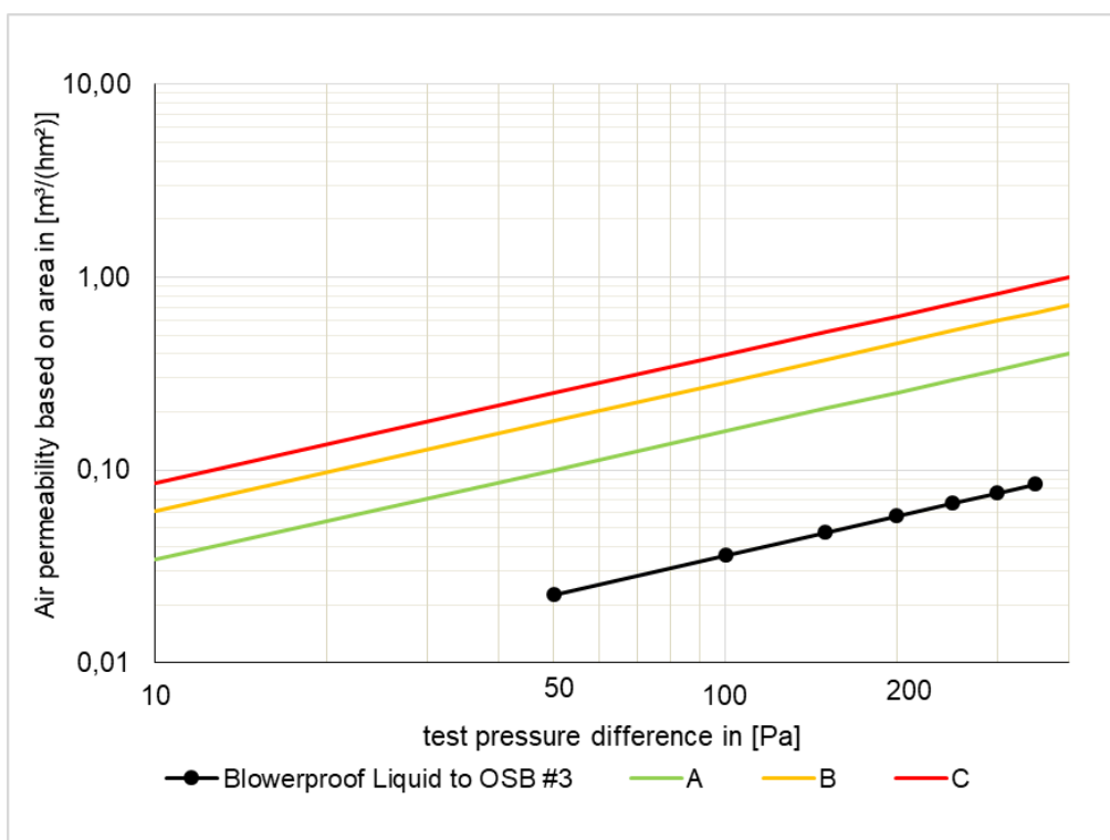
Fig. 11: Series of measurements for the sample "Blowerproof Liquid/OSB #3".. The Certification Classes A to C according to the PHI are entered in addition.
