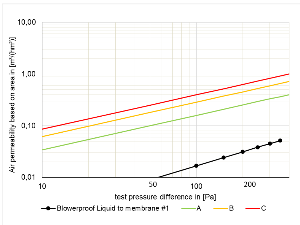
Fig. 6: Series of measurements for the sample "Blowerproof Liquid/membrane #1". The Certification Classes A to C according to the PHI are entered in addition.
