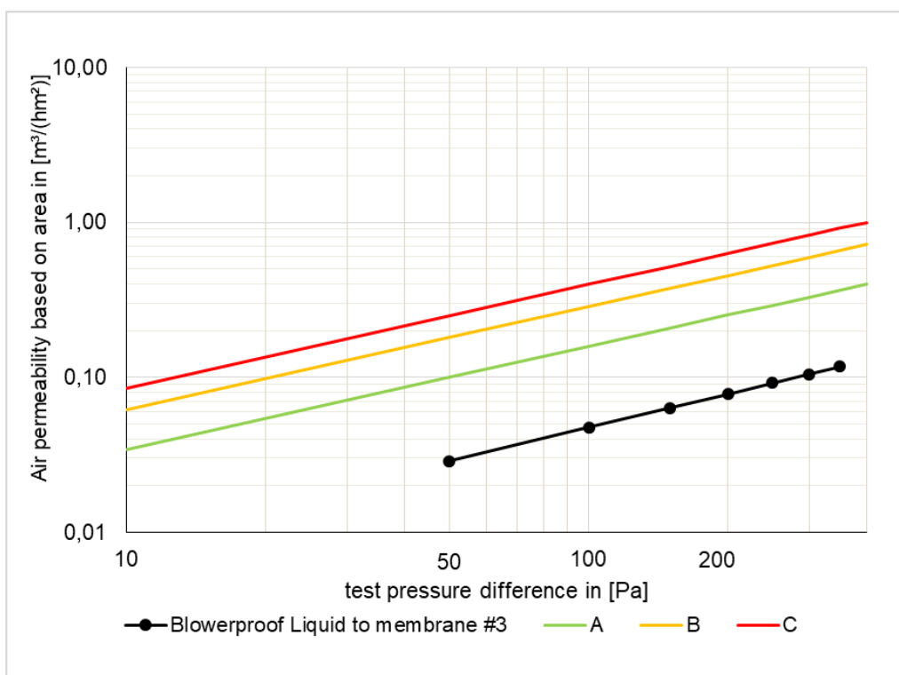
Fig. 8: Series of measurements for the sample "Blowerproof Liquid/membrane #3" The Certification Classes A to C according to the PHI are entered in addition.
