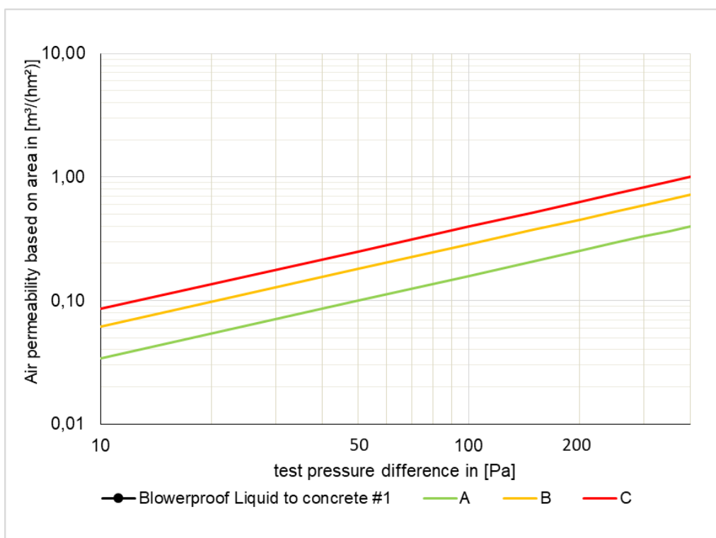
Fig. 12: Series of measurements for the sample "Blowerproof Liquid/concrete #1".. The Certification Classes A to C according to the PHI are entered in addition.
