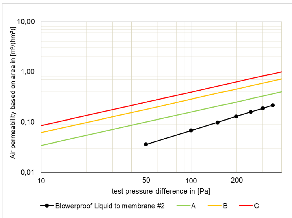
Fig. 7: Series of measurements for the sample "Blowerproof Liquid/membrane #2". The Certification Classes A to C according to the PHI are entered in addition.
