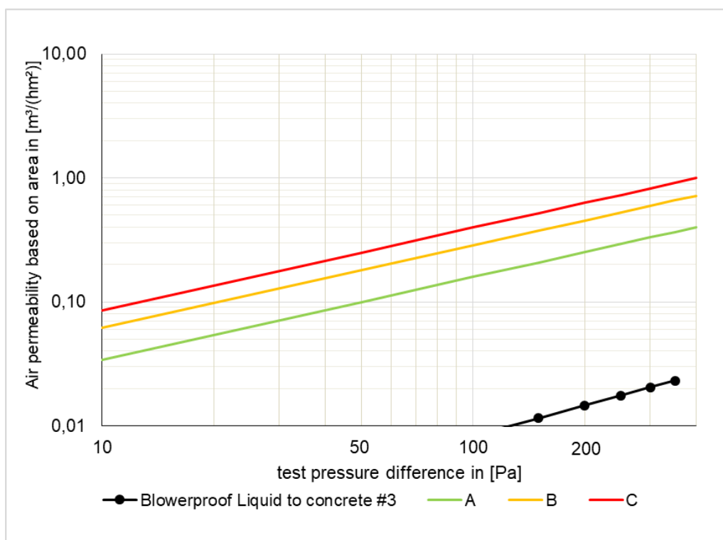
Fig. 14: Series of measurements for the sample "Blowerproof Liquid/concrete #3". The Certification Classes A to C according to the PHI are entered in addition.
